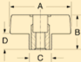
Threaded Insert Thru Hole
